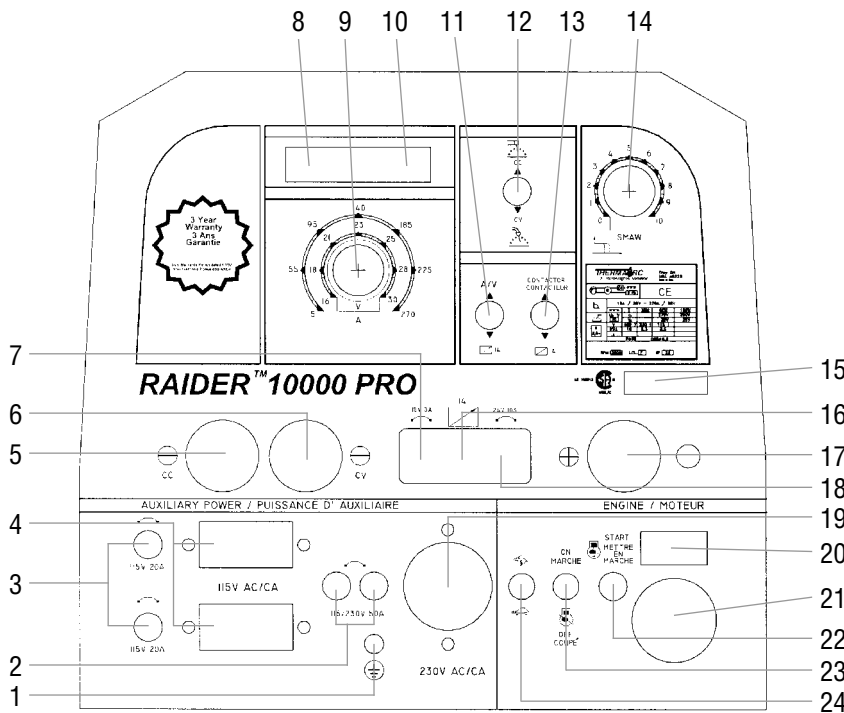
Front Panel
