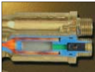
Built-in flashback arrestors prevent flashbacks
